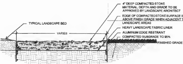
CRUSHED STONE/GRAVEL PATHWAY SECTION
